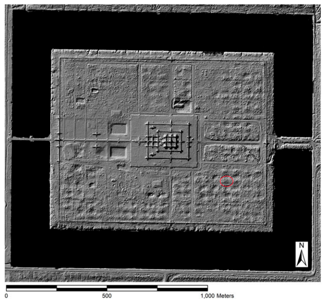
Fig. 2. LIDAR image of formal grid system across Angkor Wat enclosure with location of mound S1E2M1 circled. Digital terrain image courtesy of Khmer Archaeology Lidar Consortium.
